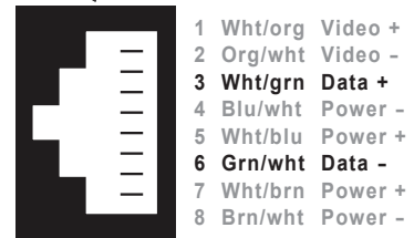
PVD Camera Port Pinout
